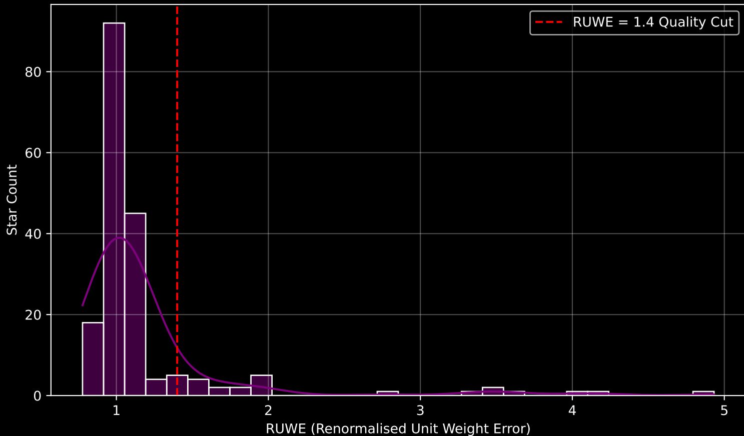
GAPOGEE DR17 Field [074+49_MGA] RUWE Distribution (n= 185)
