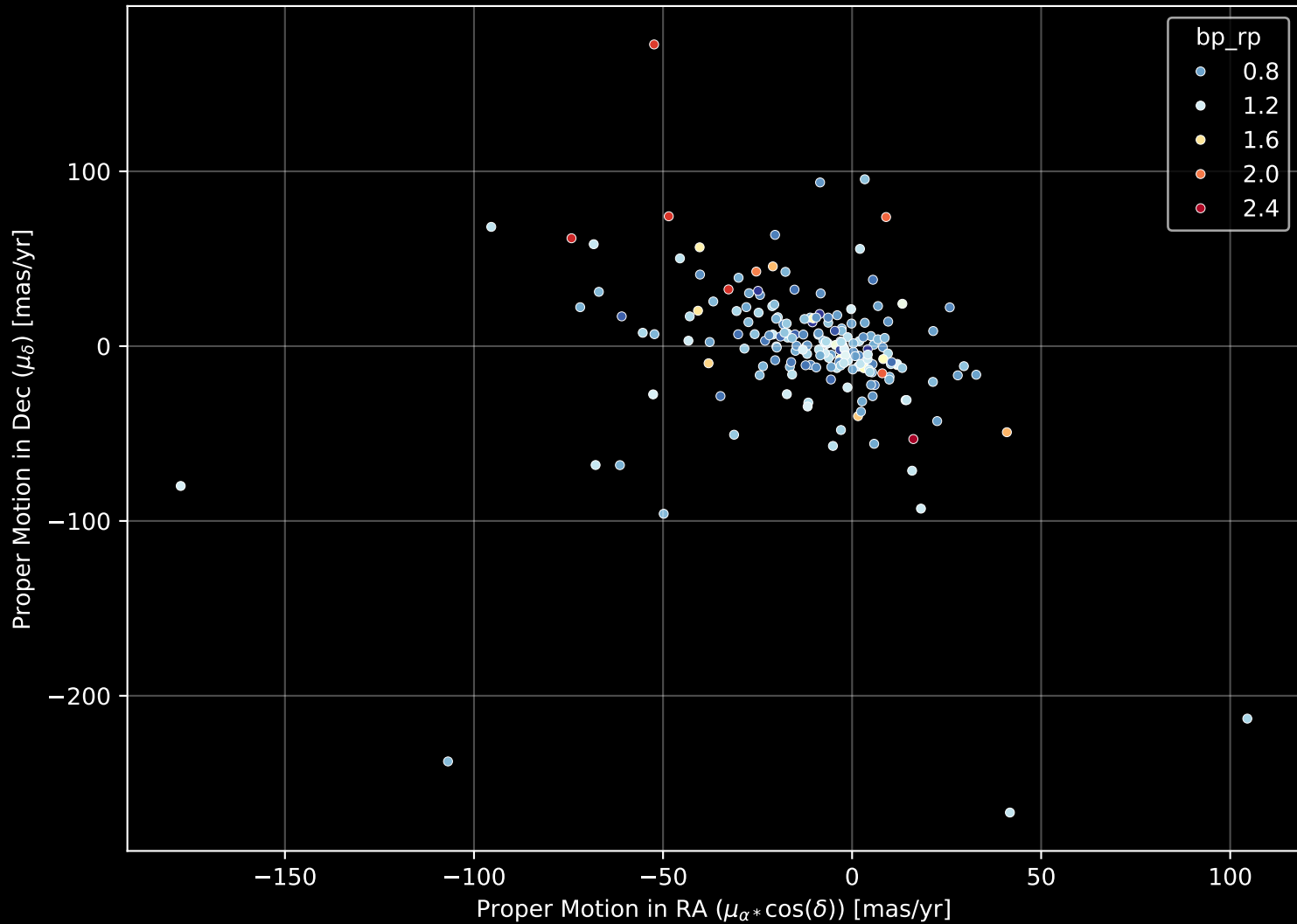
APOGEE DR17 Field: [074+49_MGA] Proper Motion Diagram (n= 197)
