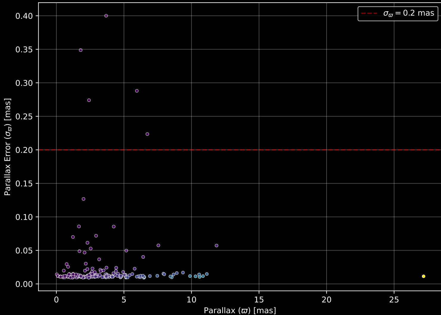
APOGEE DR17 Field: [074+49_MGA] Parallax Quality (n= 197)
