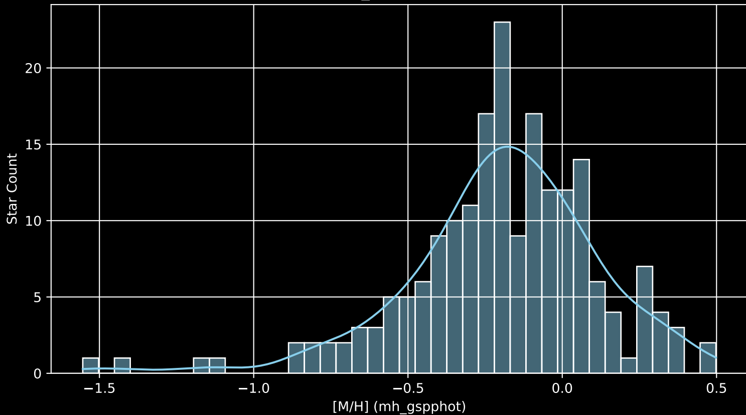
APOGEE DR17 Field: [074+49_MGA [M/H] (mh_gspphot) (n= 195)
