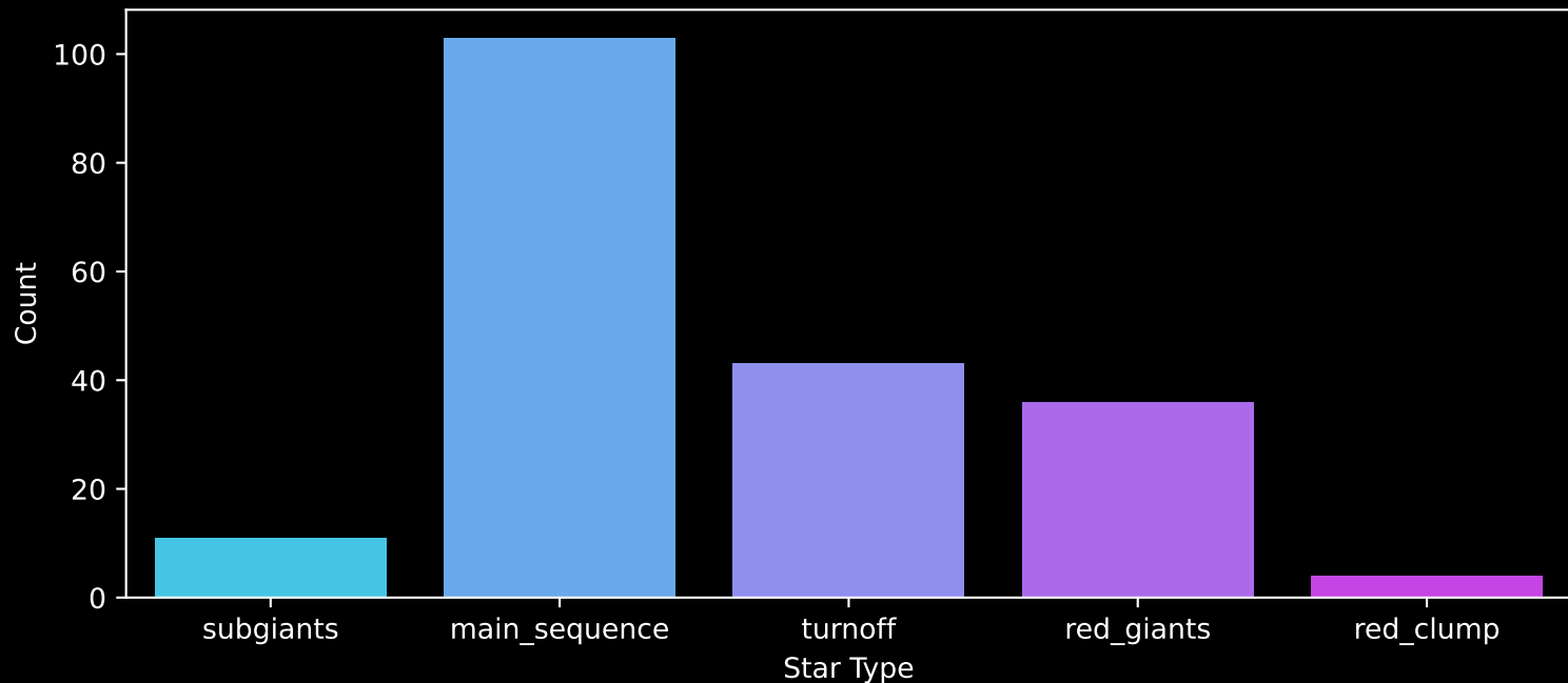
APOGEE DR17 Field: [074+49_MGA] Count plot of Star Type
