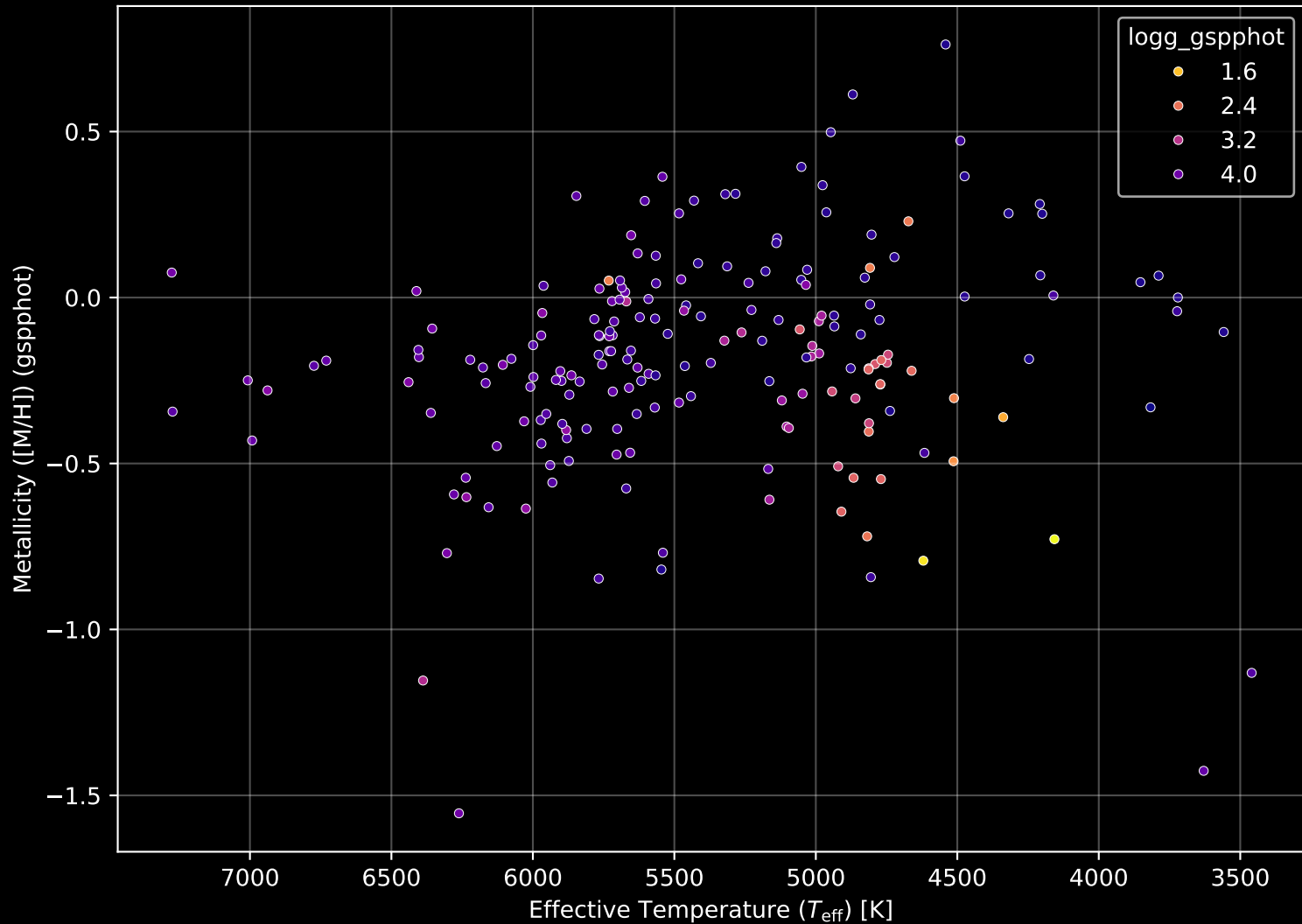
APOGEE DR17 Field: [074+49_MGA] Stellar Population Parameters (n= 197)
